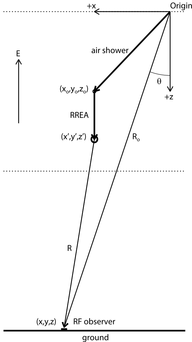
Figure 1. Diagram showing the coordinate system used in this study for the case of an upward electric field.
