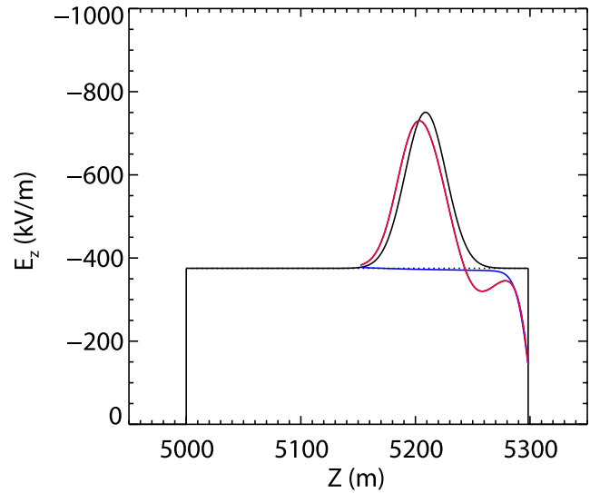
Figure 11. Same as Figure 10, except the thundercloud electric field is directed downward.
