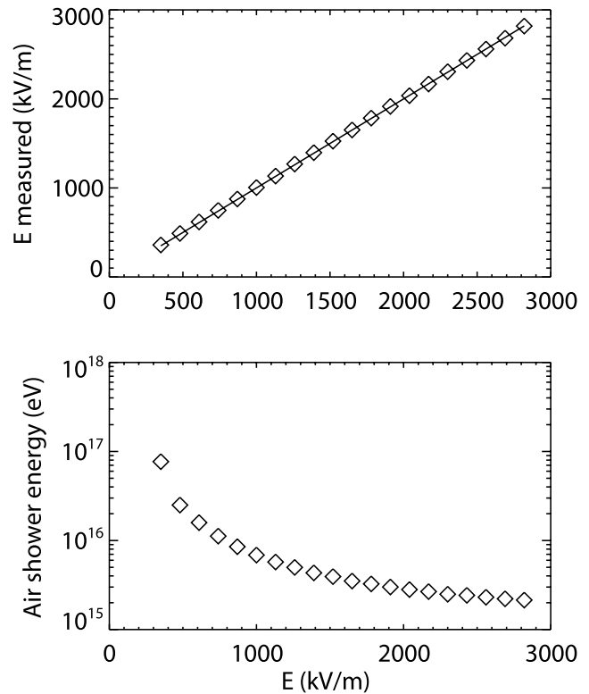
Figure 12. (top) The average thundercloud electric field that would be measured remotely versus the actual average electric field. The solid line shows unit slope. The simulation used air showers incident at 45^\circ with the antenna located on the ground where the core strikes. The thundercloud electric fields are all directed upward, and 10 avalanche lengths were used. The energy of the air shower for each electric field strength was assumed to be large enough so that the RF pulse could be well measured down to 10% of its peak value. (bottom) The minimum air shower energy required to produce measurable ( >1 mV/m) RF pulses on the ground.
