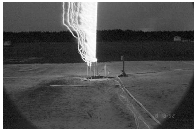
Figure 3. A photograph of the experimental site and triggered lightning S0013. The photograph was taken from the SATTILF trailer.
