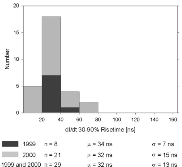
Figure 12. Histograms of current derivative risetimes.
