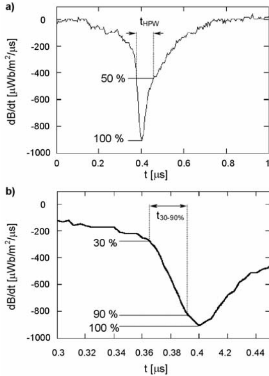
Figure 25. Magnetic field derivative at 15 m of return stroke 6 of flash S9933 on a) 1 \mu s and b) 0.15 \mu s timescales. Half-peak width and 30–90% risetime measurements are illustrated in a) and b), respectively.
