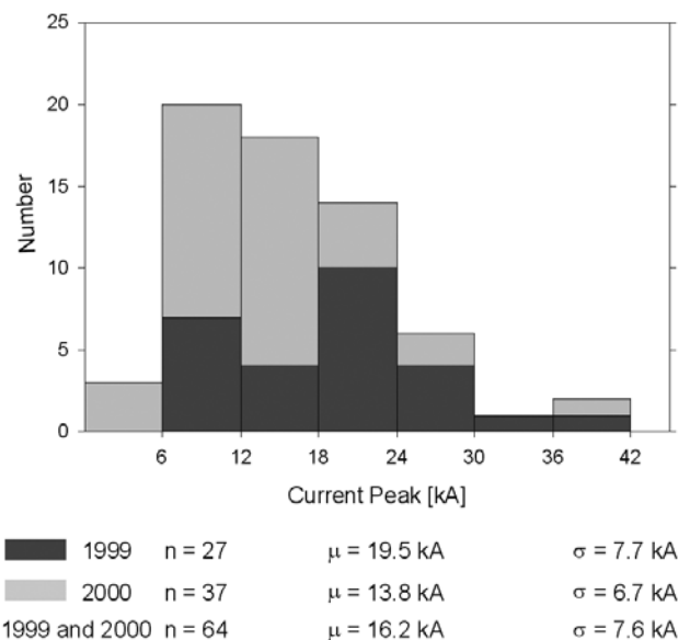
Figure 8. Histograms of current peaks. Data for 1999 and 2000 are shown stacked.
