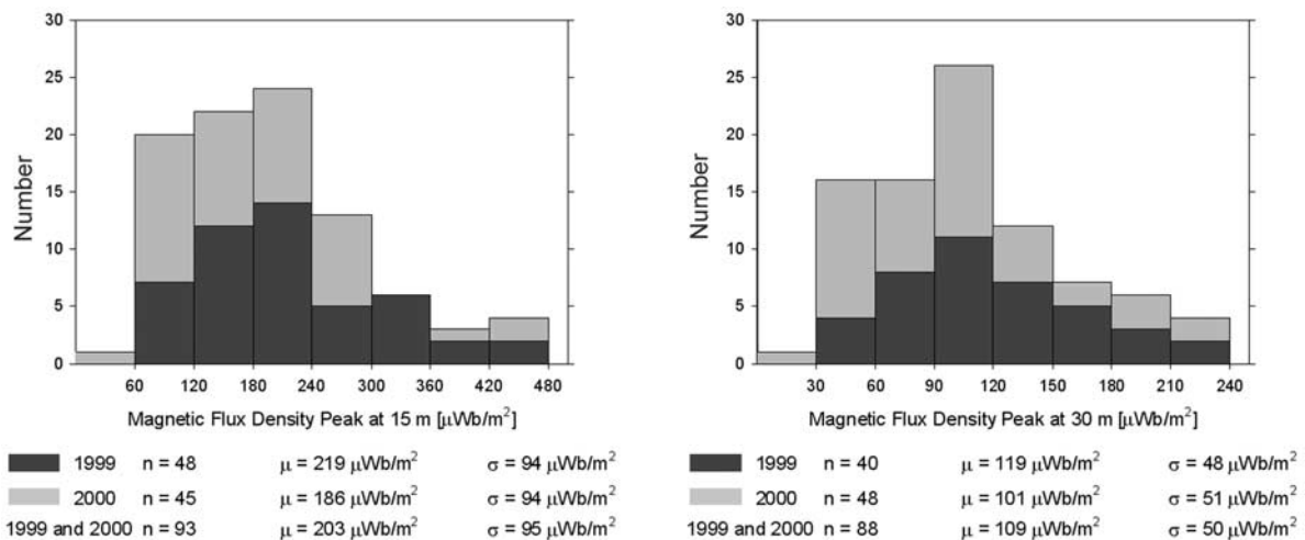
Figure 22. Histograms of magnetic flux density peaks.
