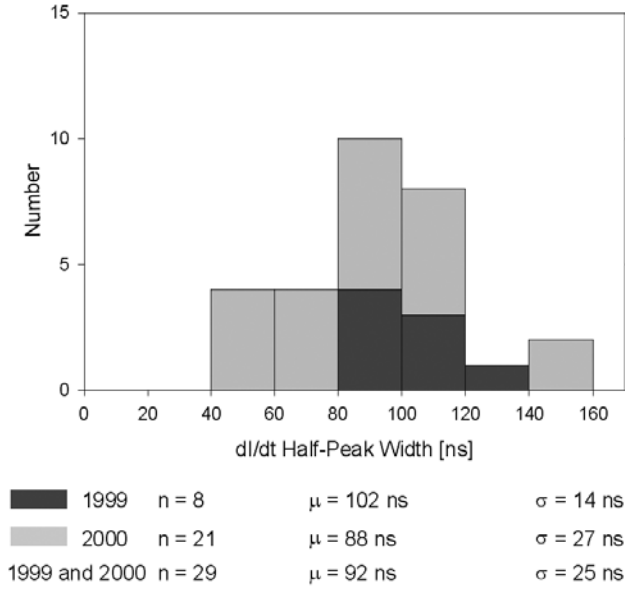
Figure 13. Histograms of current derivative half-peak widths.
