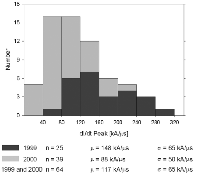
Figure 11. Histograms of dI/dt peaks. The dI/dt peaks from the 1999 experiment were obtained both from directly measured current derivative waveforms and differentiated current waveforms. The dI/dt peaks from the 2000 experiment were obtained from directly measured current derivative waveforms only.
