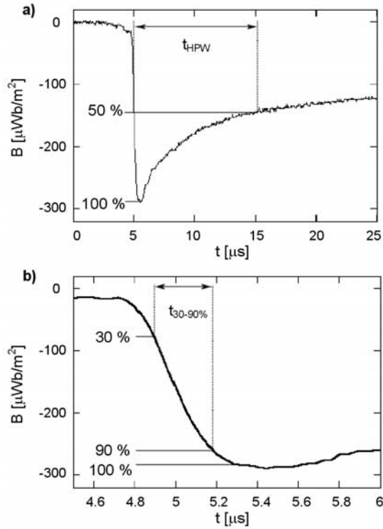
Figure 21. Magnetic field at 15 m of return stroke 3 of flash S9918 on a) 25 \mu\text{s} and b) 1.5 \mu\text{s} timescales. Half-peak width and 30–90% risetime measurements are illustrated in a) and b), respectively.
