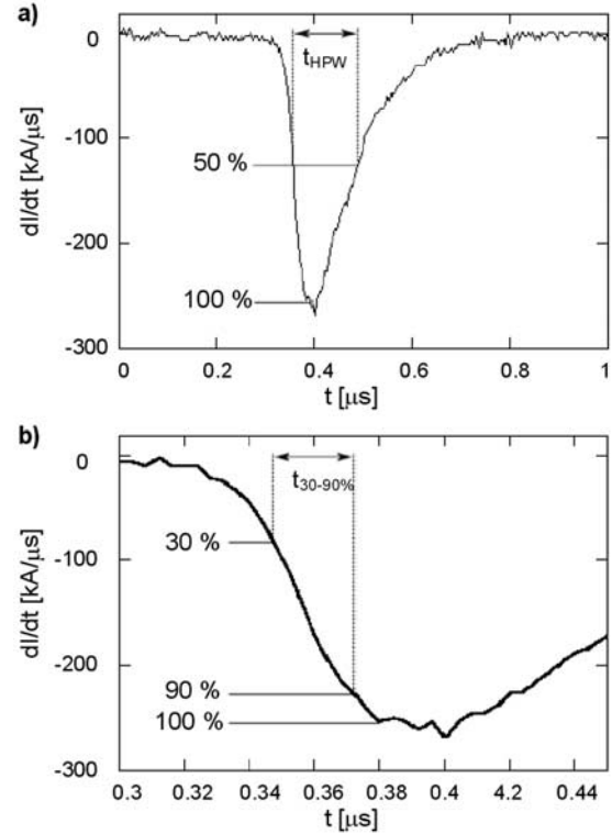
Figure 7. Current derivative record of return stroke 1 of flash S9934 on a) 1 \mu s and b) 0.15 \mu s timescales. Half-peak width and 30–90% risetime measurements are illustrated in a) and b), respectively.
