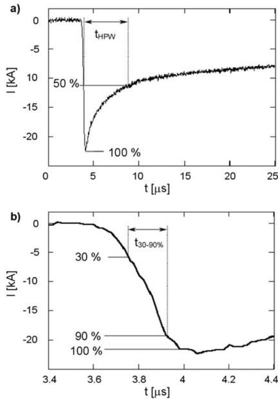
Figure 6. Current record of return stroke 2 of flash S9930 on a) 25 \mu s and b) 1 \mu s timescales. Half-peak width and 30–90% risetime measurements are illustrated in a) and b), respectively.
