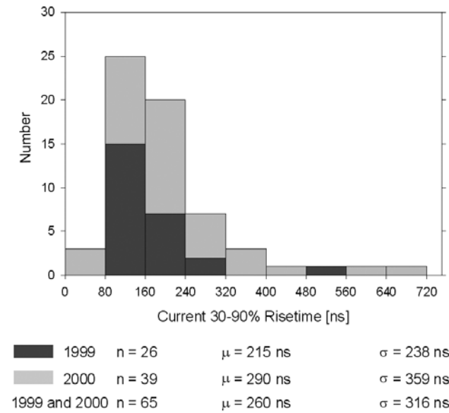
Figure 9. Histograms of current risetimes. Three values, 1300 ns (1999), and 1680 ns and 1750 ns (2000), are not shown in the histograms but are included in the statistics.
